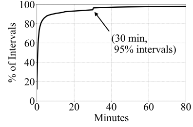
Fig. 14. Interval Distribution
